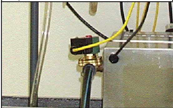
12 VDC 1/2 NPT Solenoid Valve con- nected to water supply up to 100 psi
